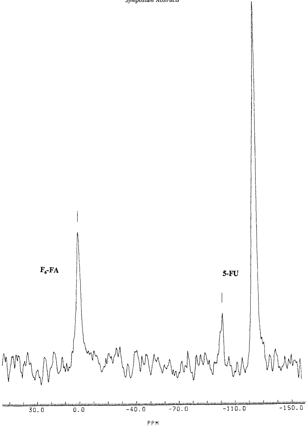
Figure 2. In vivo ^{19}\text{F} MRS of rat liver after injectoin of F 6 -FA and 5 fluorouracil (5-FU)
